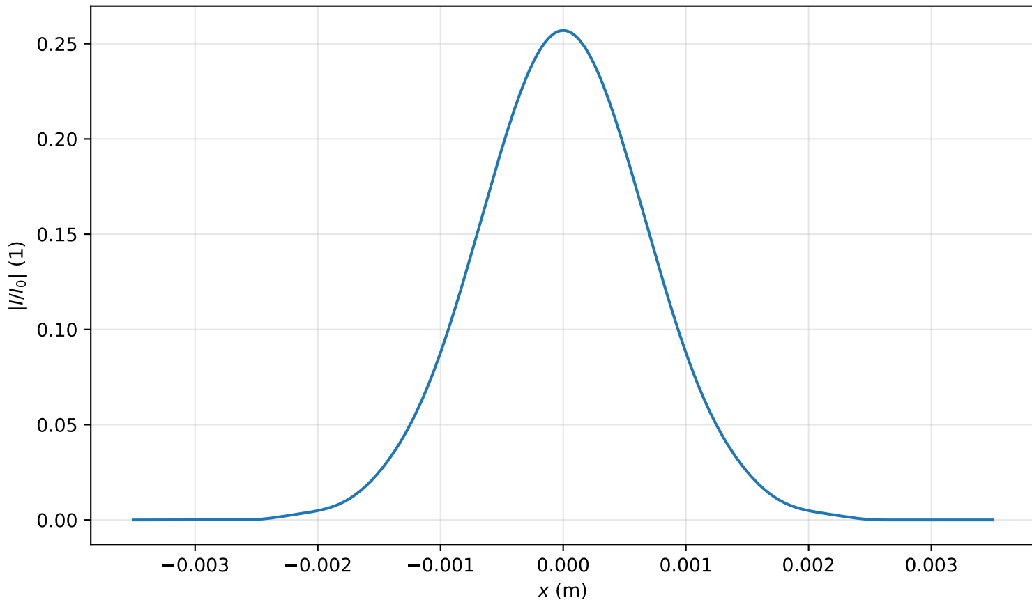
Intensity profile I(x, y = 0, z = 3.901m)/I_0 , P_{in}=0.2P_{cr} , artificial time
